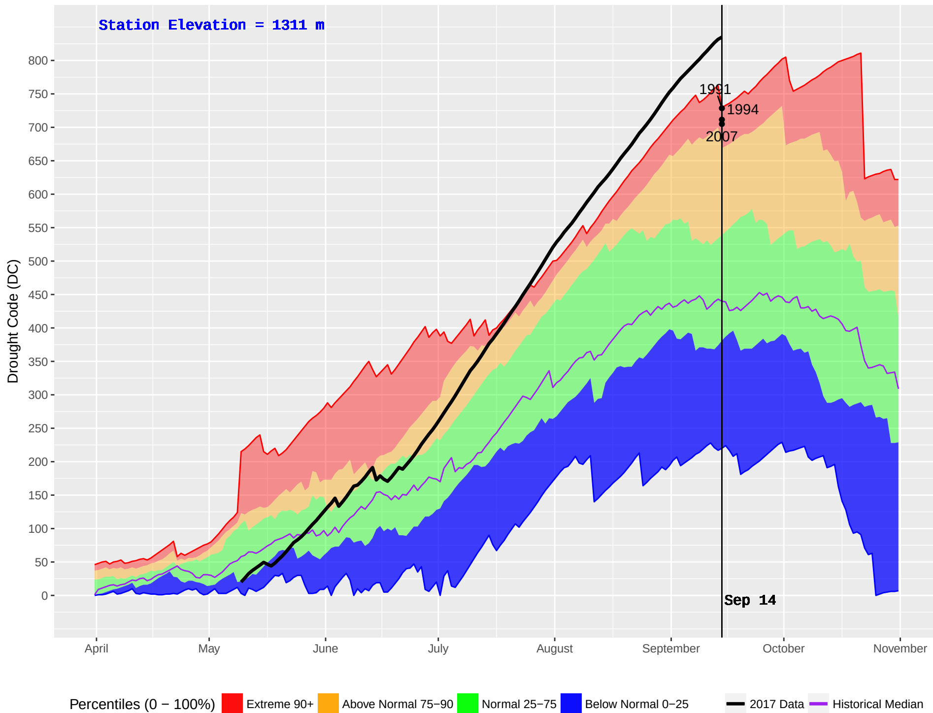
FLATHEAD 2 (418) : Historical (1986–2016) and Current (2017) Noon Drought Code (DC)
