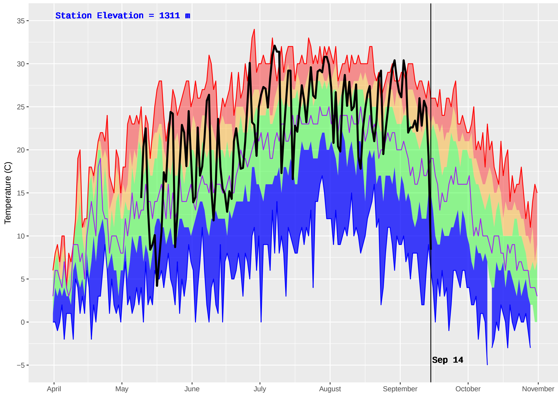
FLATHEAD 2 (418) : Historical (1986–2016) and Current (2017) Noon Temperature
