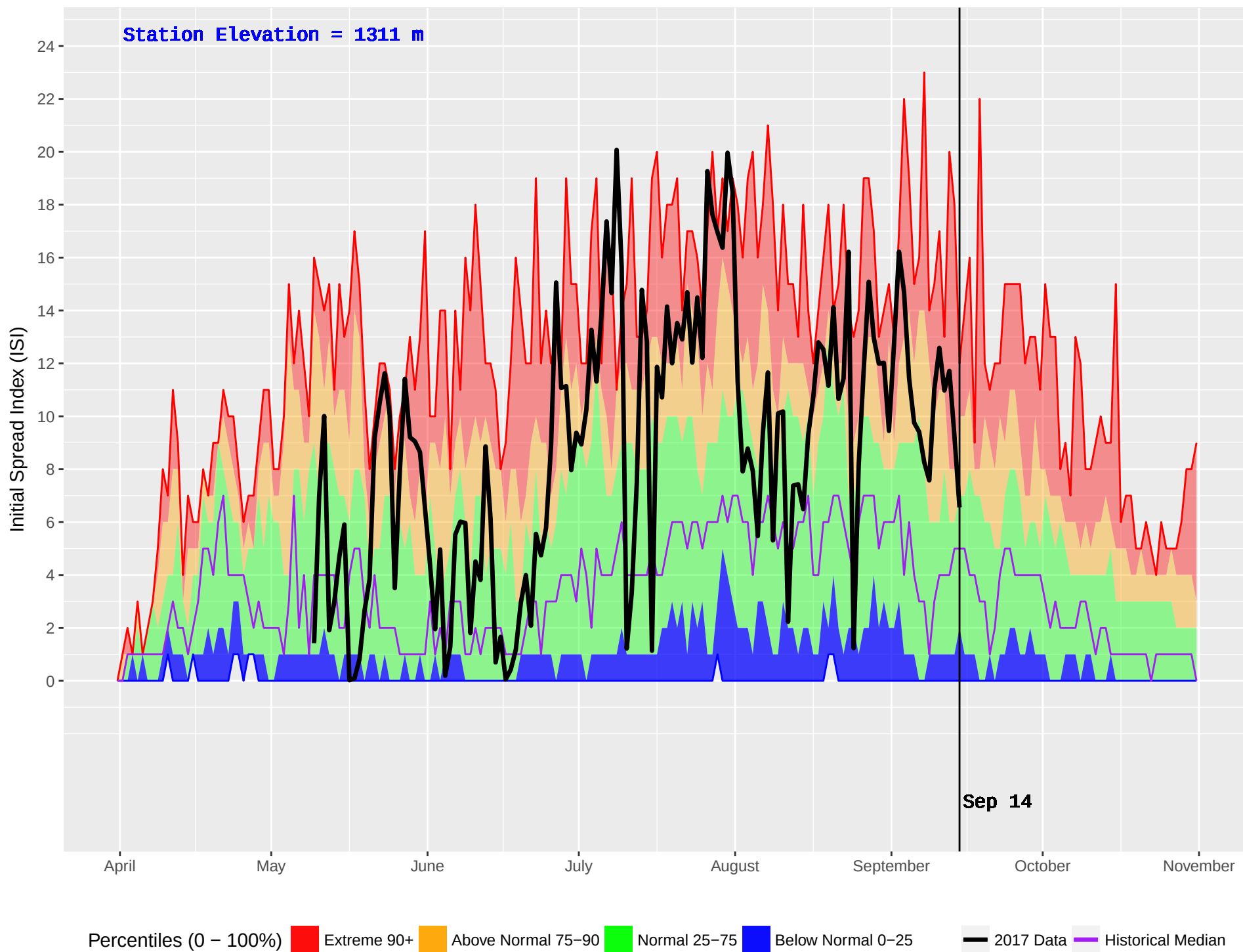
FLATHEAD 2 (418) : Historical (1986–2016) and Current (2017) Noon Initial Spread Index (ISI)
