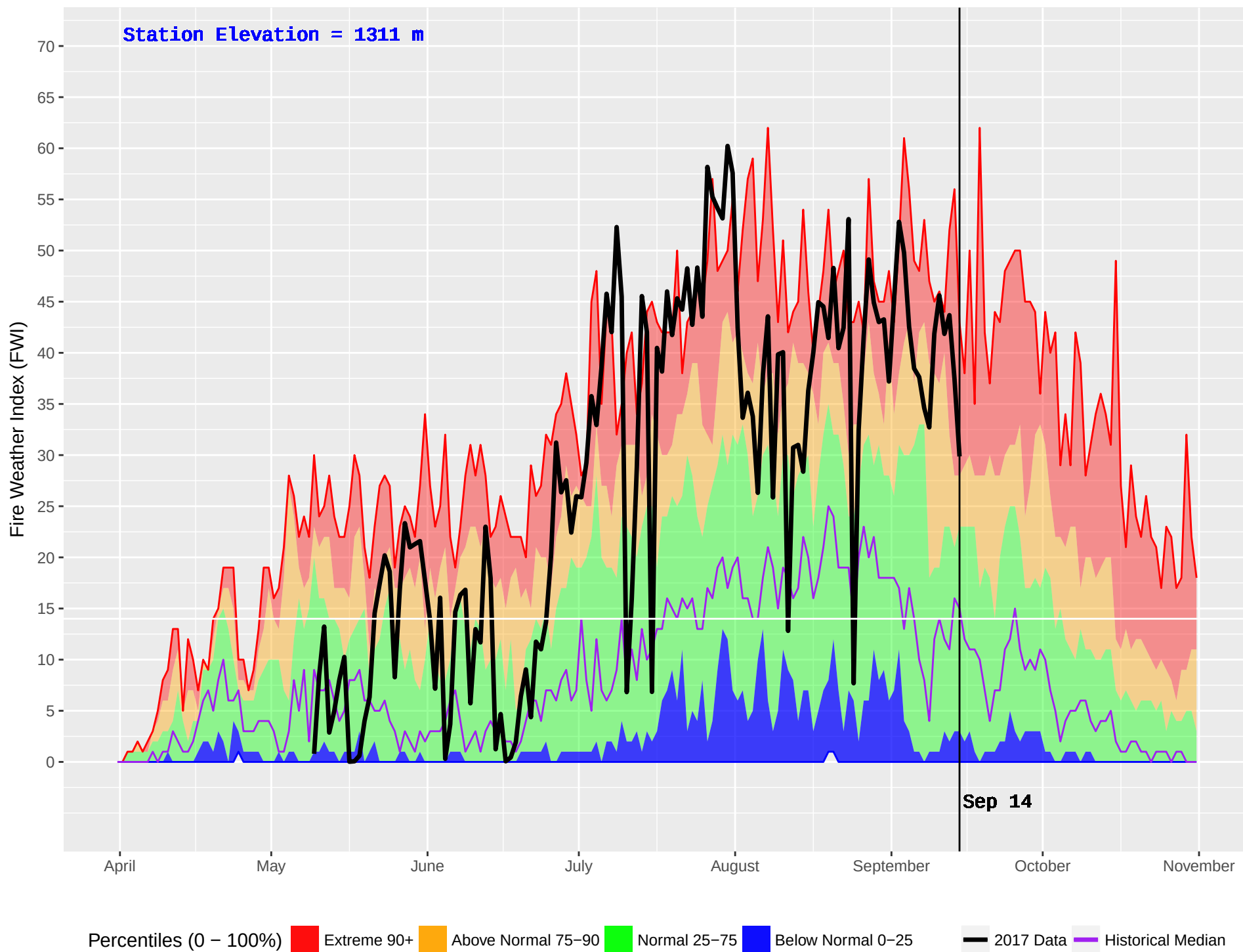
FLATHEAD 2 (418) : Historical (1986–2016) and Current (2017) Noon Fire Weather Index (FWI)
