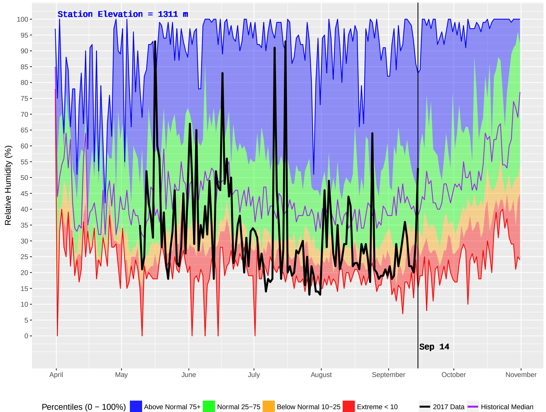
FLATHEAD 2 (418) : Historical (1986–2016) and Current (2017) Noon Relative Humidity
