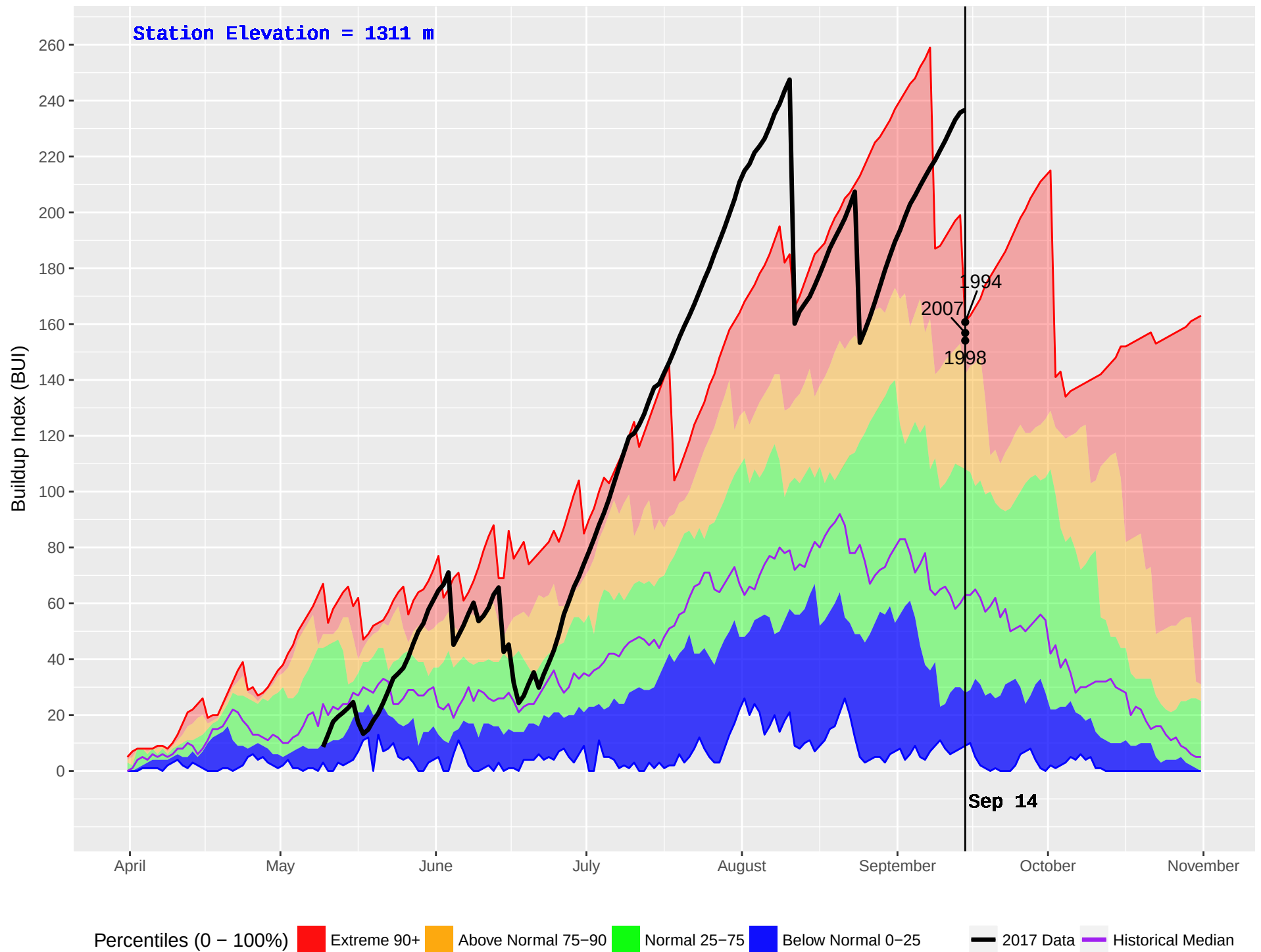
FLATHEAD 2 (418) : Historical (1986–2016) and Current (2017) Noon Buildup Index (BUI)
